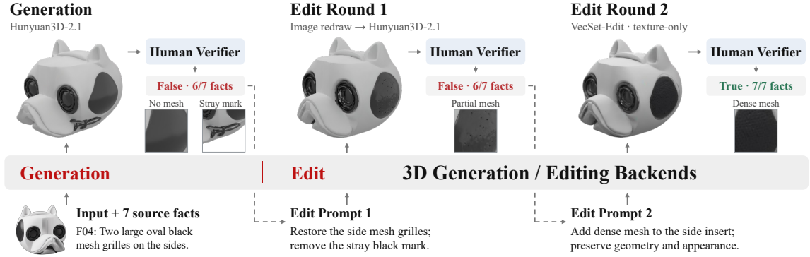
Figure 6: Human-guided 3D recursive refinement trajectory. Given the source image and target facts, initial generation exhibits a missing side grille and a surface artifact (left, 6/7 facts). A revised one eliminates the artifact but leaves the grille incomplete (middle, 6/7 facts). Subsequent edit fully restores the mesh appearance and satisfies all facts (right, 7/7 facts). Intermediate 2D conditions and masks are omitted.
