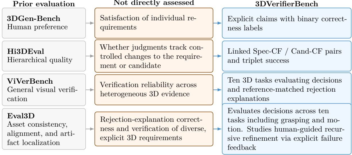
Figure 2: Evaluation scope relative to prior work. Prior work (Zhang et al., 2025a;b; 2026b; Duggal et al., 2025) emphasizes preference, hierarchical quality, general visual verification, or asset-level consistency and artifact localization. Our 3DVerifierBench targets complementary verifier-side questions through explicit requirements, controlled counterfactuals, heterogeneous 3D evidence, and verification-guided refinement.
