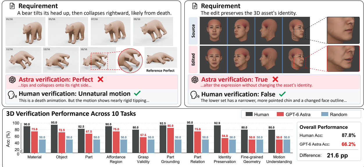
Figure 1: Even state-of-the-art MLLMs, e.g. , GPT-6 Astra, still struggle with 3D content verification. Top: Astra mistakenly accepts an unnatural rightward collapse and an identity-changing face edit. Bottom: We found that Astra is still far behind human performance across all tasks in our 3DVerifierBench. Views and text are abbreviated for display.
