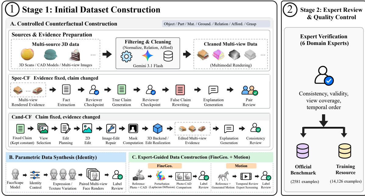
Figure 4: Our pipeline. Reviewed evidence establishes positive anchors. Spec-CF changes the requirement under fixed evidence, whereas Cand-CF changes the candidate under the original requirement. Native annotations and task-specific evidence complement these controlled mutations. Automated checks, model-assisted review, and human review together produce the benchmark.
